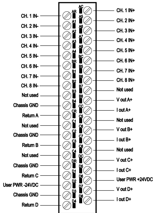
Figure 2.9 Output Screw Terminal Connector Wiring
