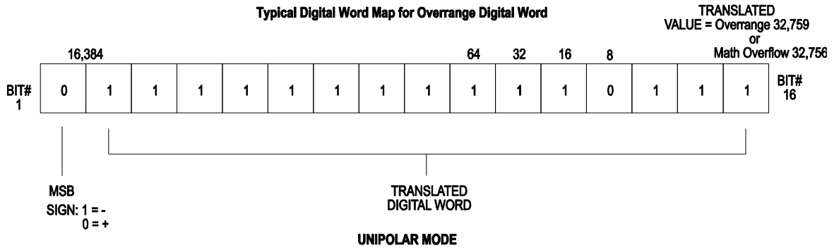
Figure 1.5 Overage Word Value (Unipolar)
