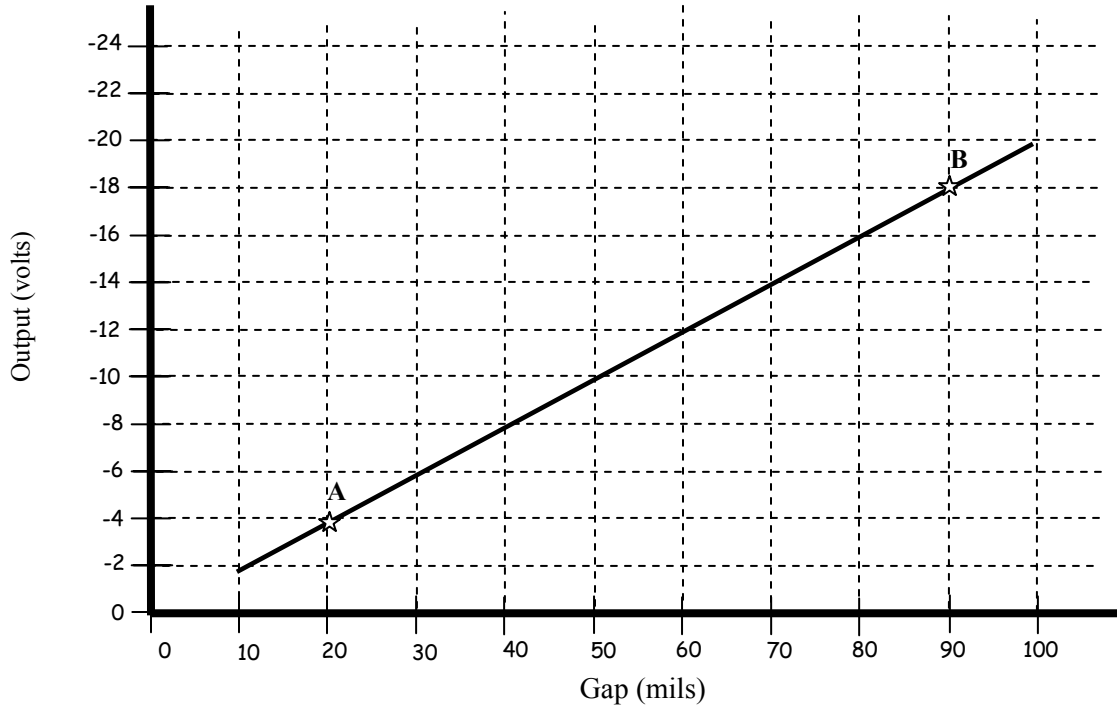
Figure 3.2. Displacement probe (200mV/mil) chart example
