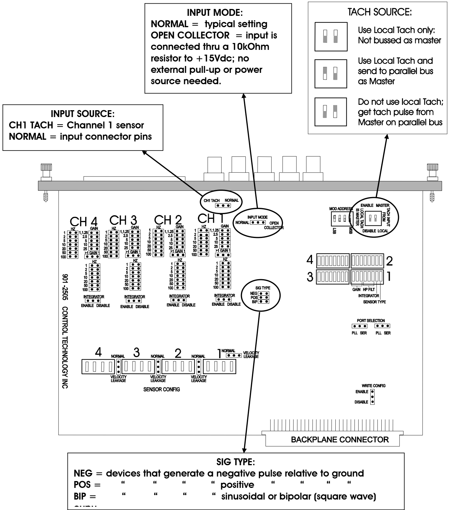
Figure 2.7. Selecting Tachometer Options
