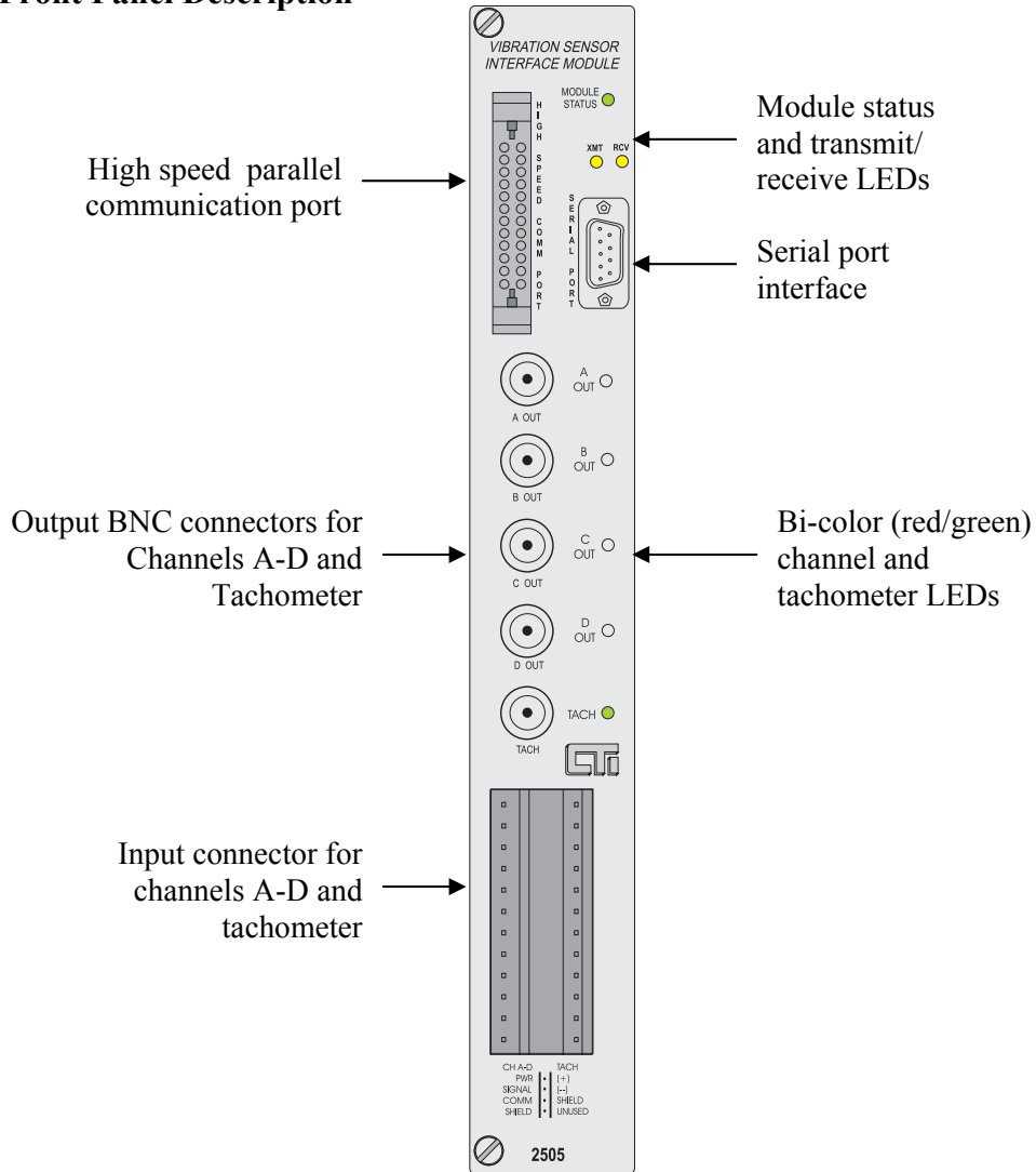
Figure 1.1. CTI 2505 Front Panel
