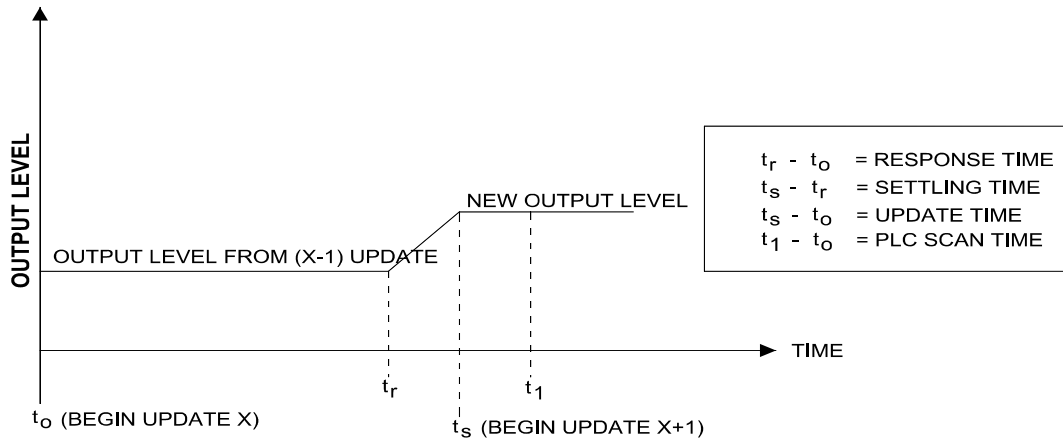
Figure 1.2. Relation of Update Time Change in Signal Input
