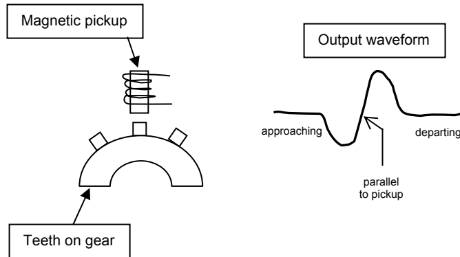
Figure 2.6. Bipolar gear tooth example
