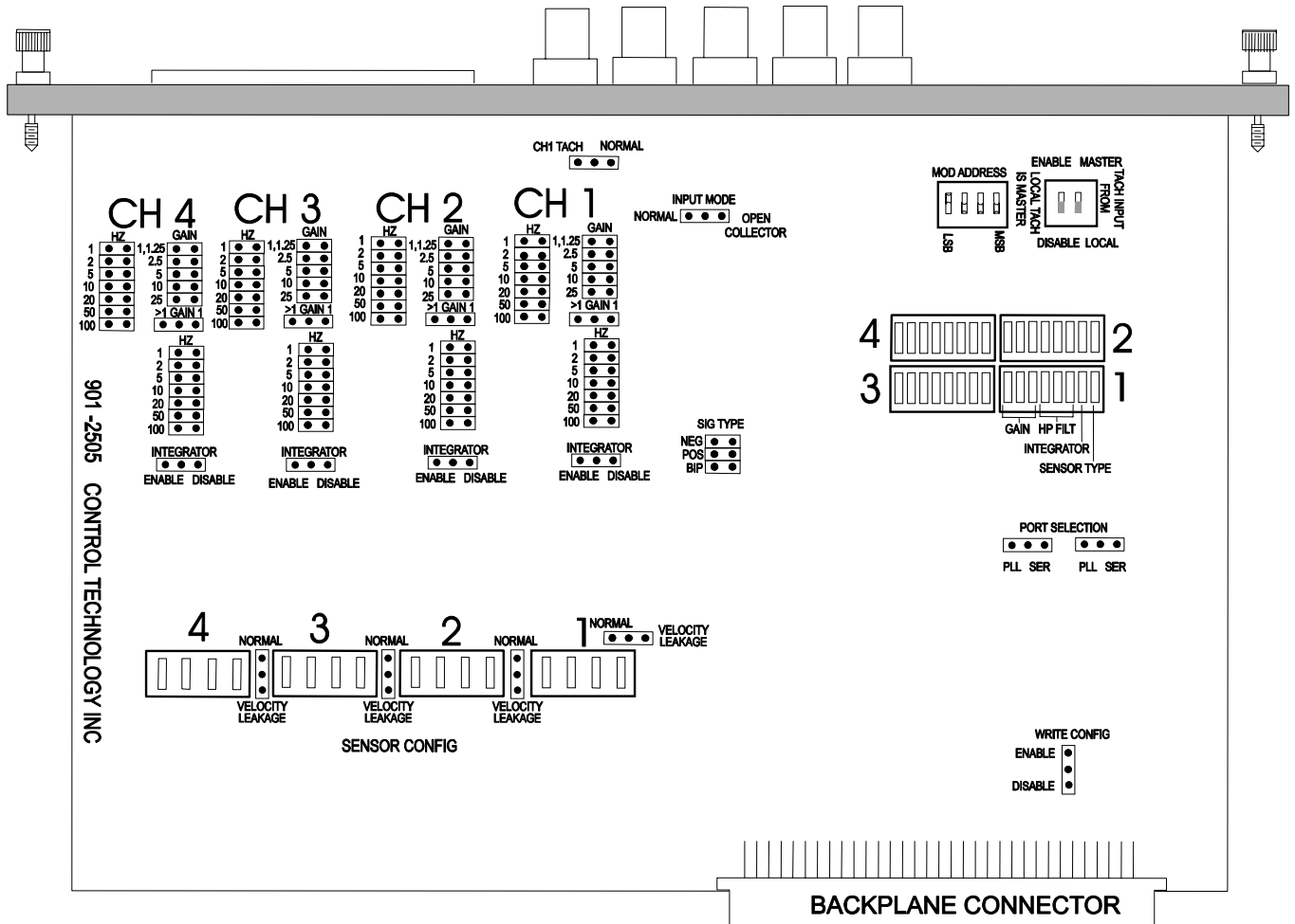
Figure 2.1. Jumper and Switch locations
