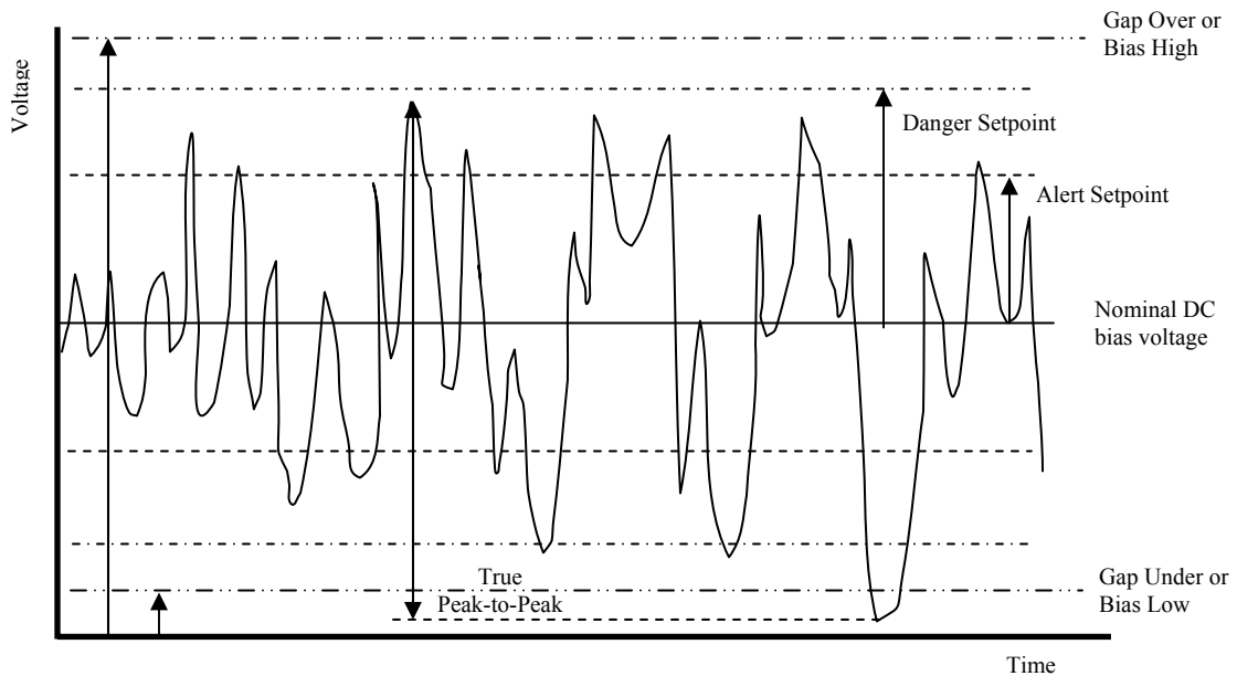
Figure 3.1. Alarm & Danger levels, Time Delay example chart
