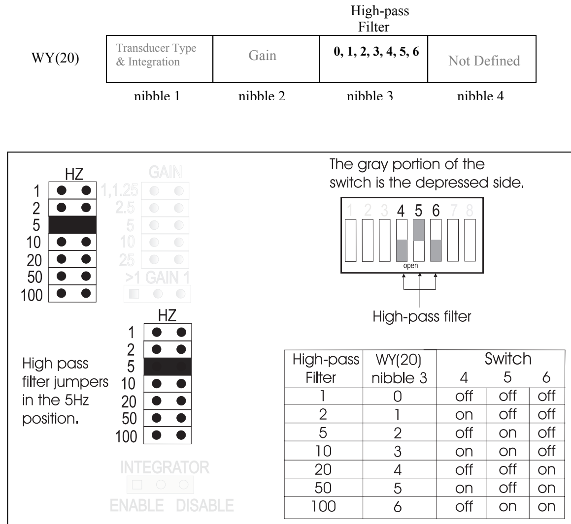
Figure 2.3. Selecting High-Pass Filter Value
