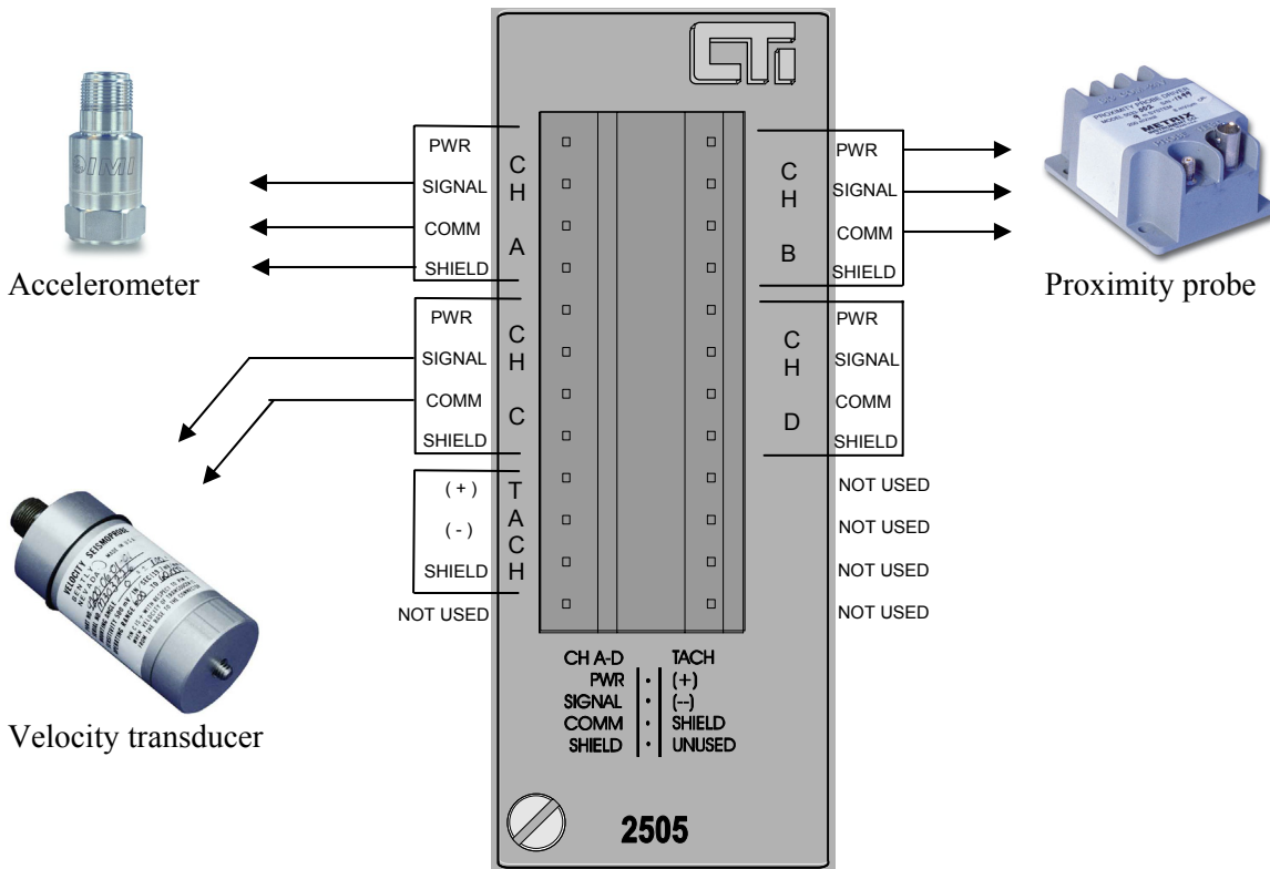
Figure 1.1.a. CTI 2505 Wiring Connector
