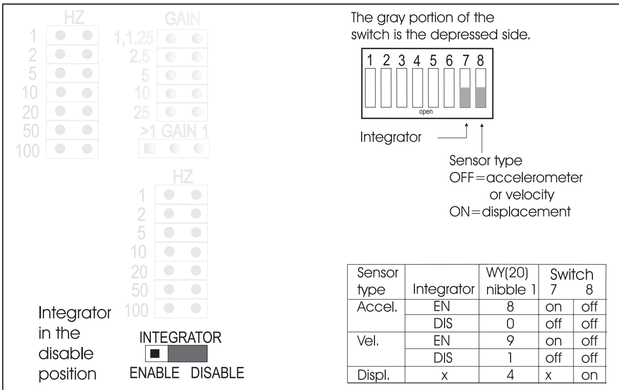
Figure 2.5. Selecting the Integration and Sensor Type
