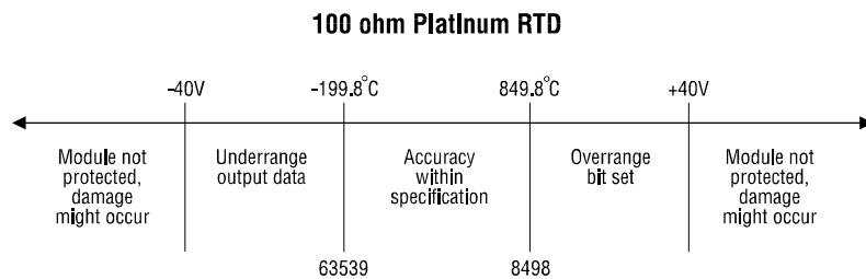
Figure 6 Effect of Temperature Input on Module Performance
