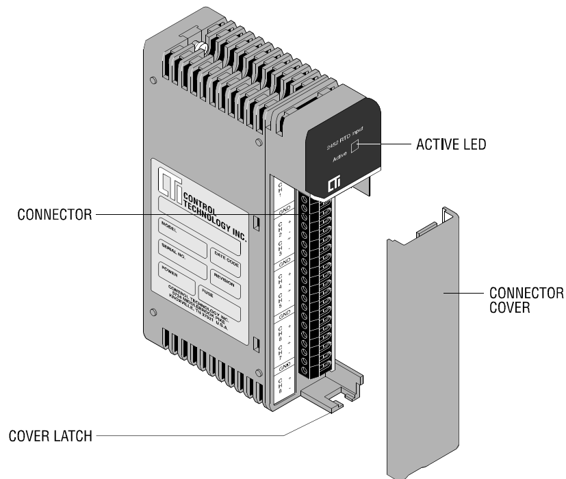
Figure 2 2452 Front Panel
