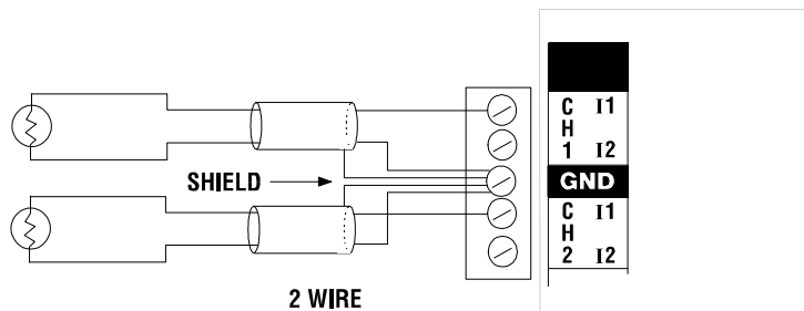
Figure 12 Wiring Example 2-Wire RTD
