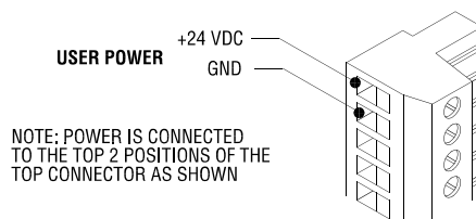
Figure 11 Power Supply Connections
