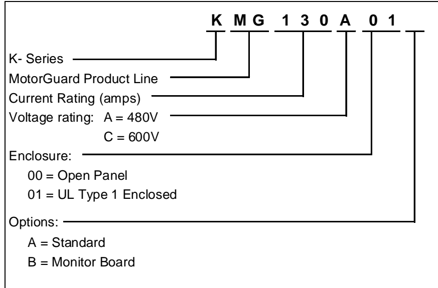
Figure 2a – MotorGuard Model Number Encoding – Industrial Version
