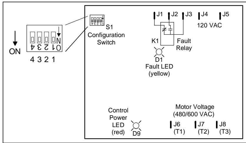
Figure 5 – Monitor Board Component Layout
