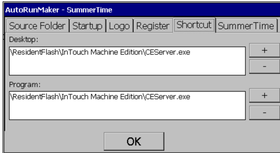
FIGURE 3: AUTO RUN MAKER - ITCMGR IS REMOVED
