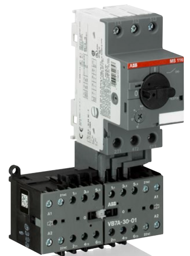
With manual motor starter
