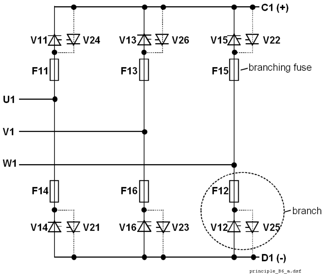
Bridge configuration D5 to D7
