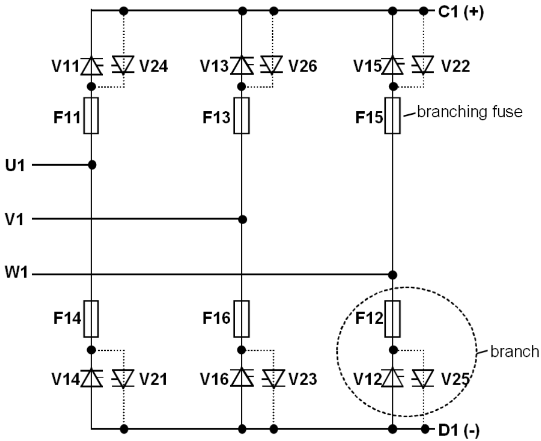
Bridge configuration D5 to D7
