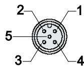
Adam M12-5 male connector. (Note that some models have 4 or 8 pins instead.)
