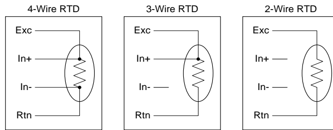
Figure 1: RTD Terminals
