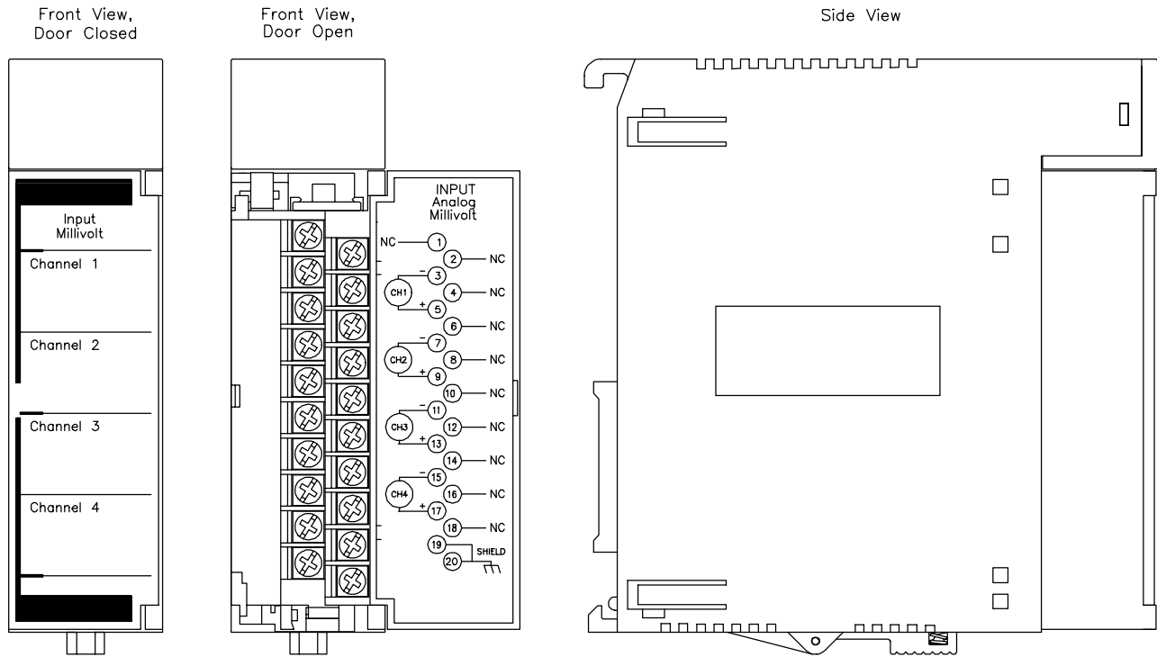
Figure 1 – HE693ADC406 / 409 Module
