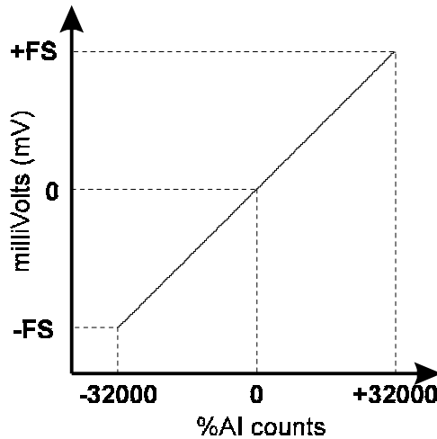
Figure 4 – Input Scaling
