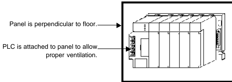
Figure 1.1 – PLC Positioning for Adequate Ventilation
