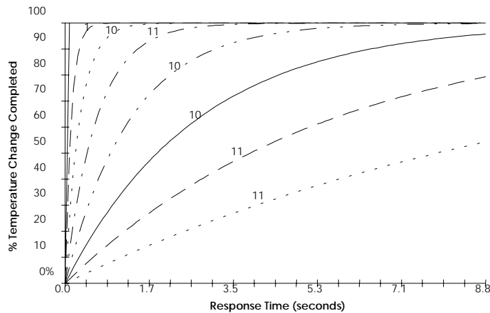
Figure 3 - Digital Filtering
