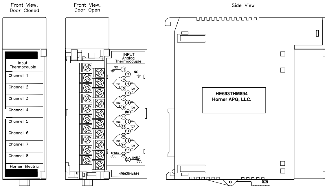
Figure 1 – HE693THM894 Module
