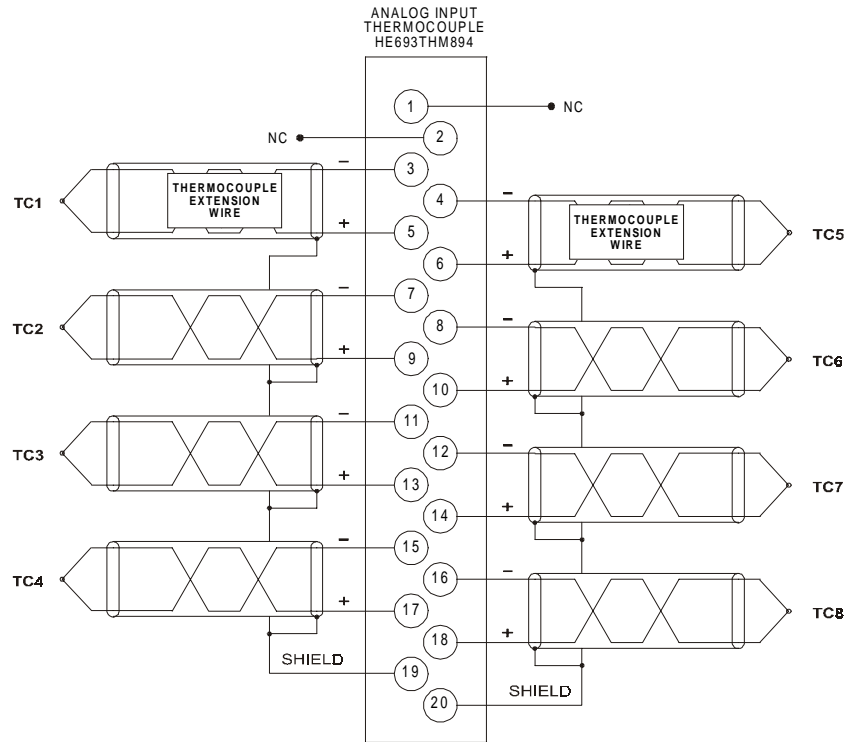
Figure 4 – THM 894 Wiring
