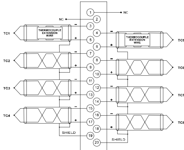
Figure 4 – THM 895 Wiring
