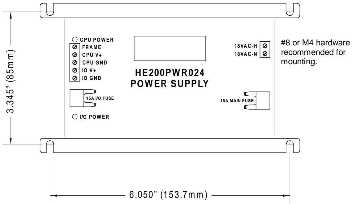
Figure 1 – HE200PWR024 Module
