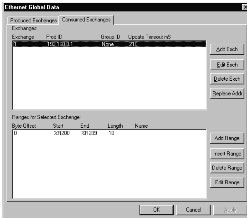
Figure 6.20 – Configured Consumed Exchange 1 - Node 2
