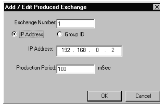
Figure 6.8 – Creating Produced Exchange 1 - Node 1
