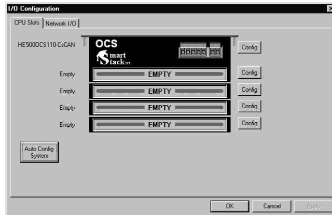
Figure 3.2 – I/O Configuration Dialog – OCS Models With User-Installable Ethernet
