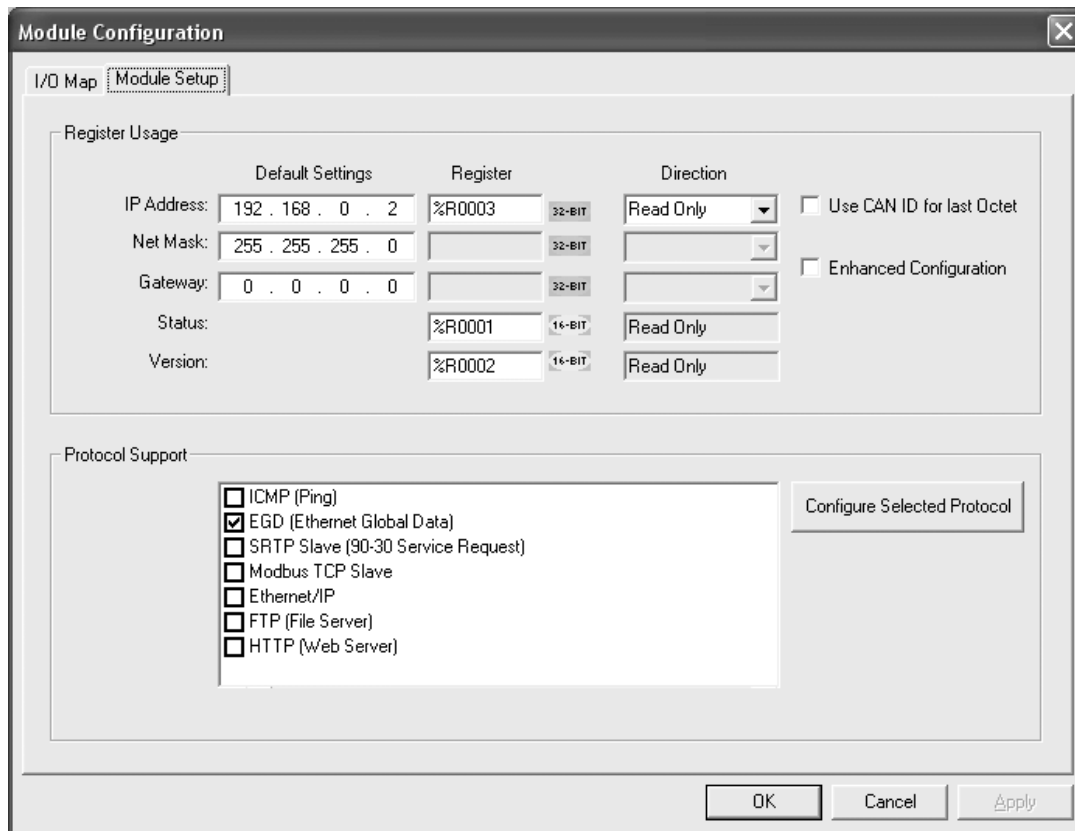
Figure 6.14 - Ethernet Module Configuration - Node 2
