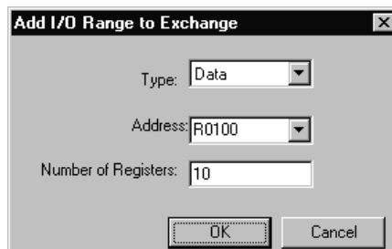
Figure 6.9 – Produced Exchange 1 Data Block Definition – Node 1
