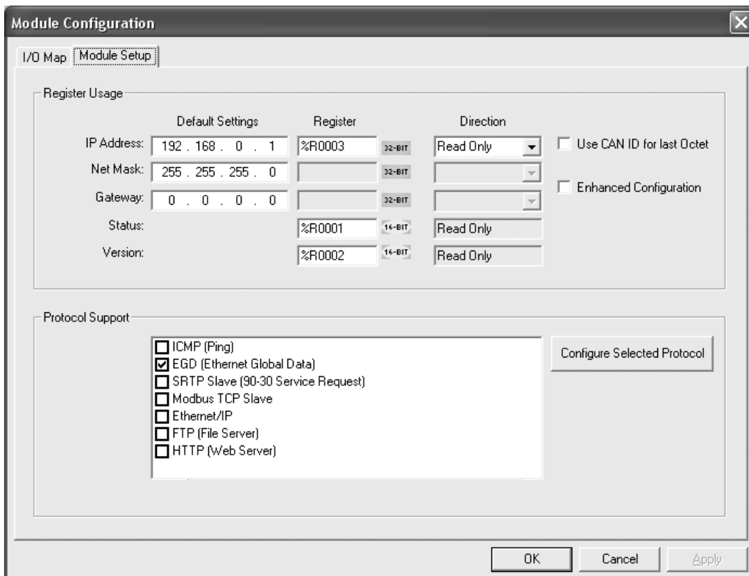
Figure 6.7 - Ethernet Module Configuration - Node 1
