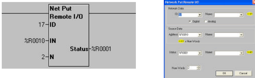
Figure 2 - Put Remote I/O Function Block and Parameter Screen
