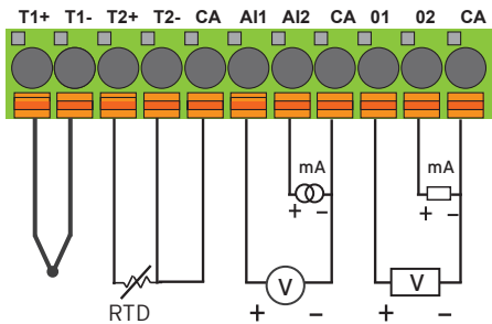
J1: CA terminals are internally connected together and isolated from BUS.
