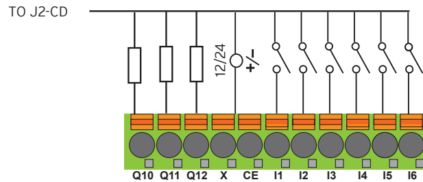
J4: X has no internal connection. CE is isolated from BUS.
