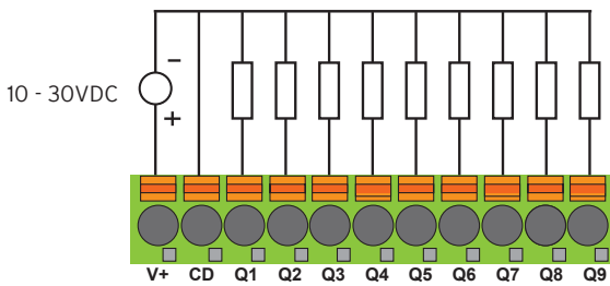
J2: V+ and CD are isolated from BUS.
