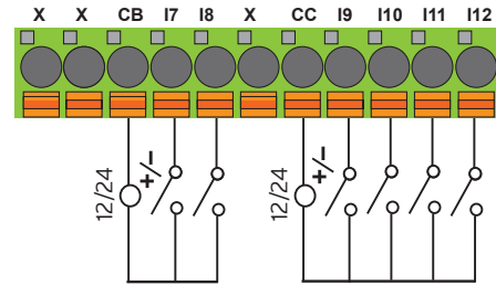
J3: X has no internal connection. CB and CC terminals are isolated from each other and BUS.
