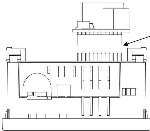
Figure 1 - Removing Back Cover of the XLE
