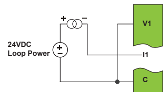
20mA Analog In - Not Self-Powered
