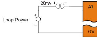
20mA Analog In - Not Self Powered
