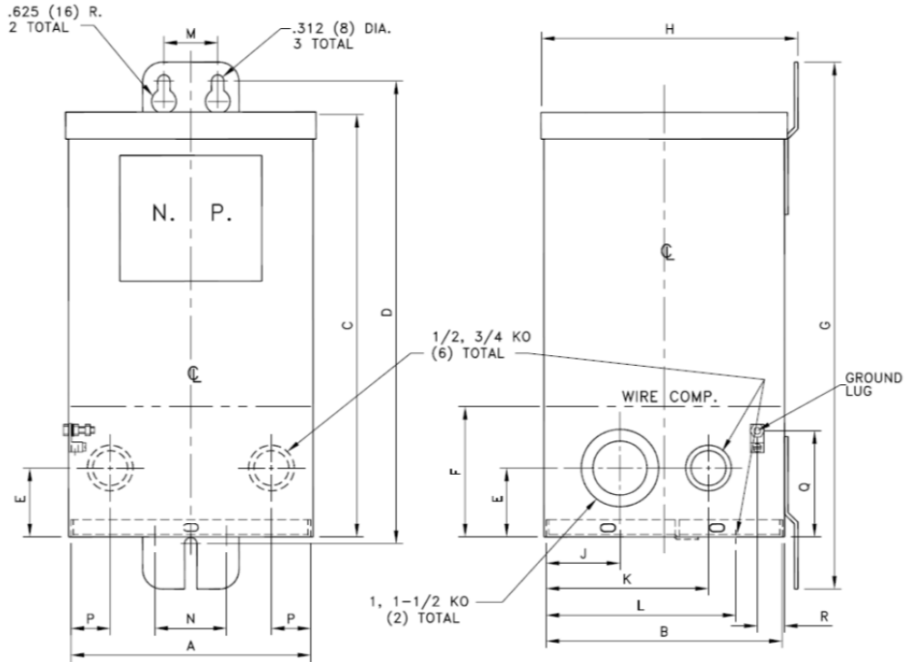
DIMENSIONS IN inches (mm)
