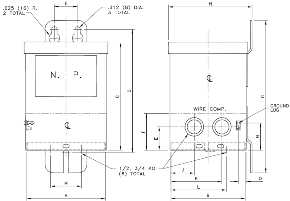
DIMENSIONS IN inches (mm)
