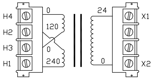
CONNECTION DIAGRAM
