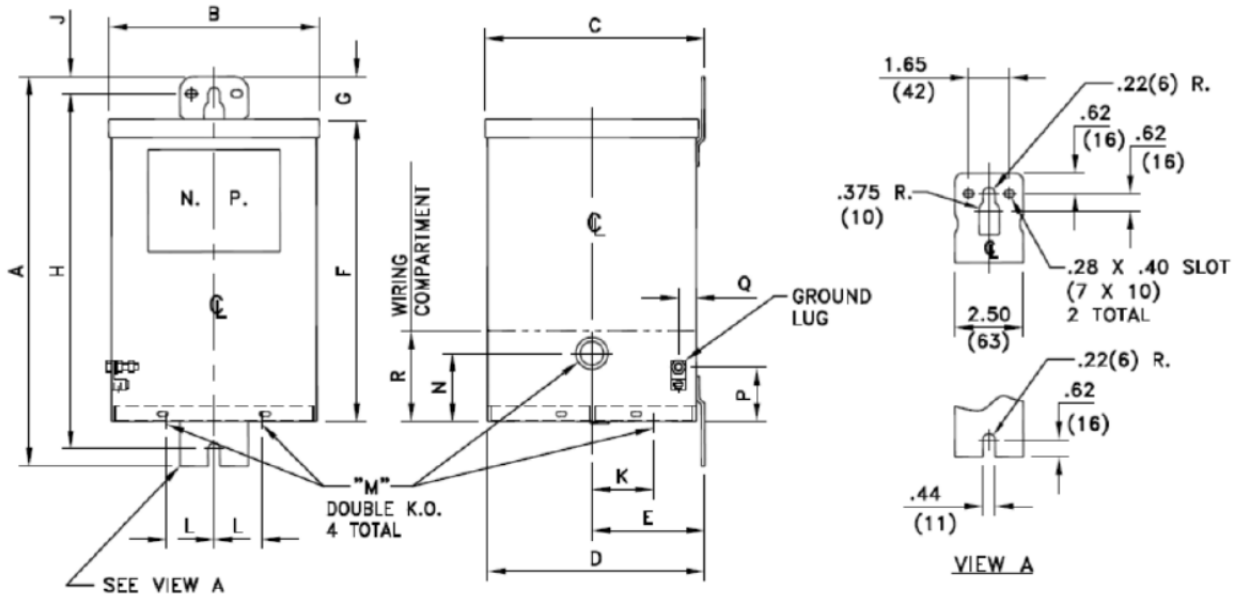
DIMENSIONS IN in(mm)
