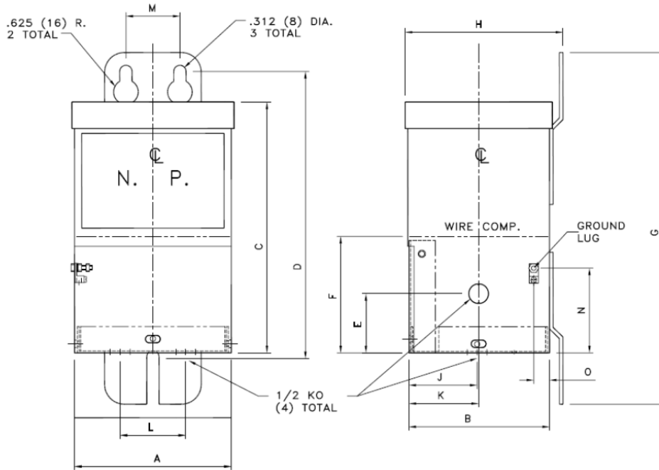
DIMENSIONS IN in(mm)
