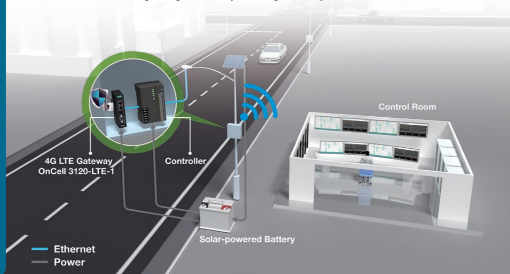
OnCell 3120-LTE-1 Series LTE cellular gateway with serial connectivity
