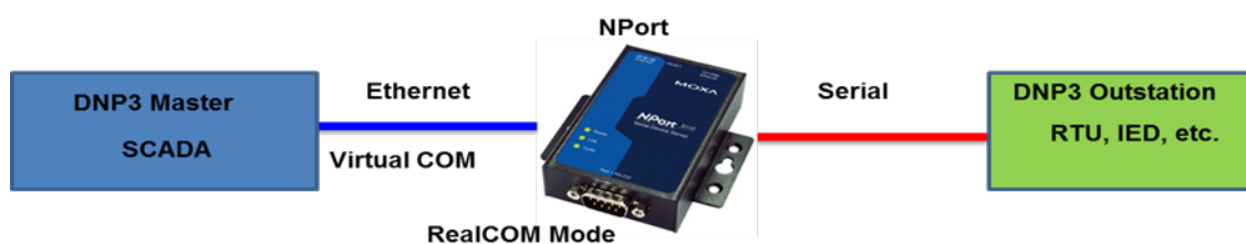
Figure 1: System Topology
