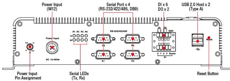
Rear View
