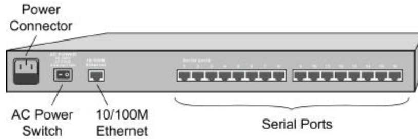
Figure 1-3. 16-Port NPort Server Pro Rear Panel (DE-303)
