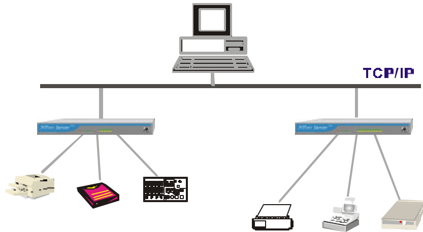
Figure 2-2. Single-Host Mode using two NPort Server Pros
