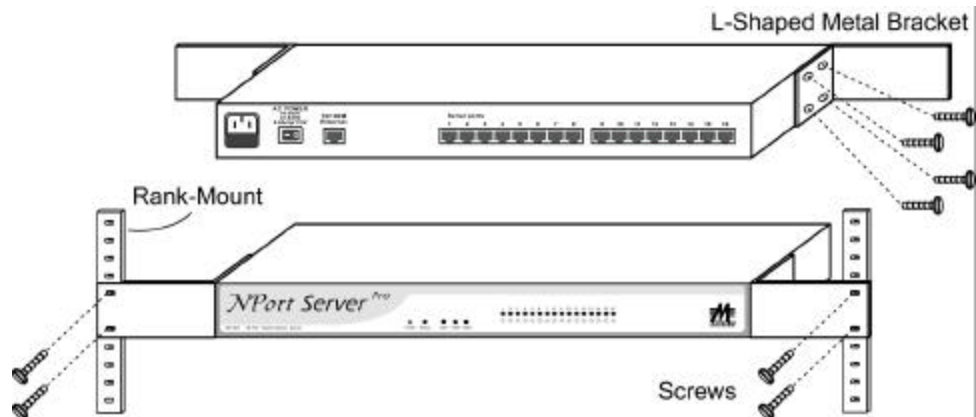
Figure 2-5. Rack Mount
