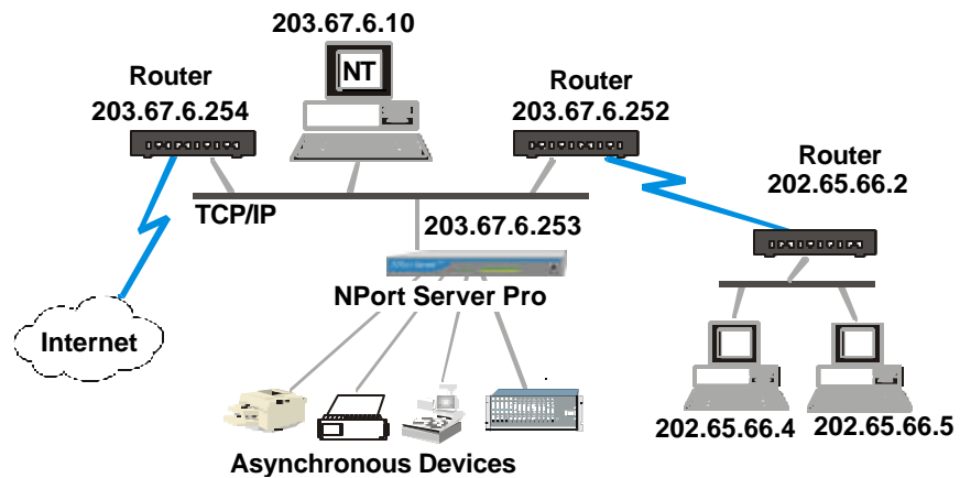
Figure 6-4. Scheme for NPort Server Pro connecting to the Intranet and Internet.
