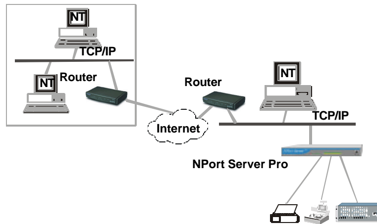
Figure 6-1. A remote control link diagram
