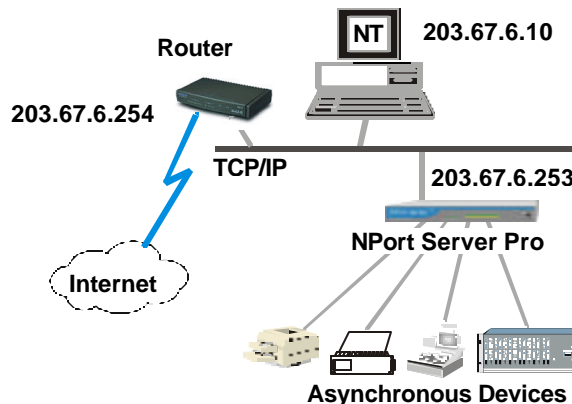
Figure 6-3. Scheme for LAN with NPort Server Pro connecting to the Internet
