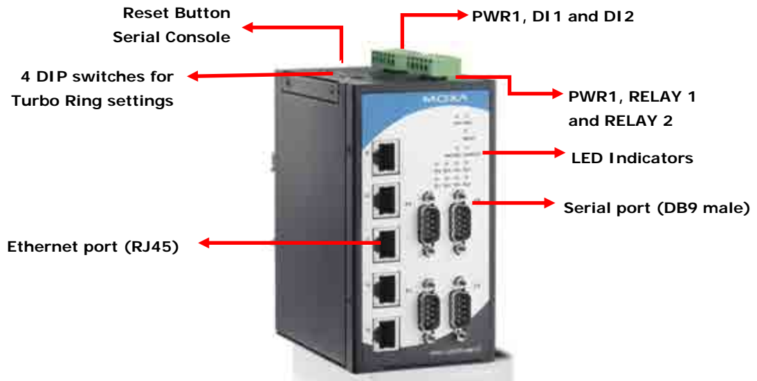
NPort S8455I Series
