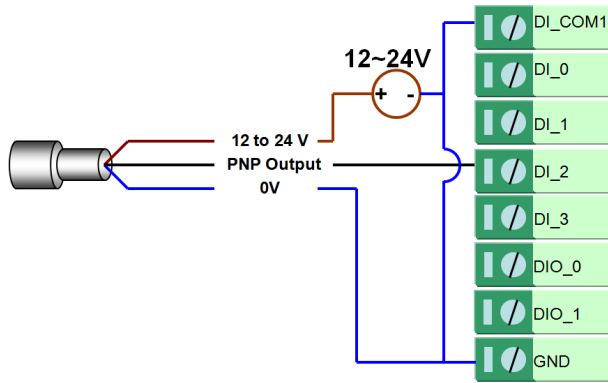
PNP Type Sensors Connection
