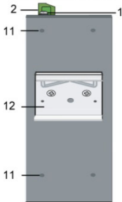
Rear Panel View
