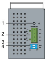
Rear Panel View
