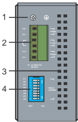
Rear Panel View
