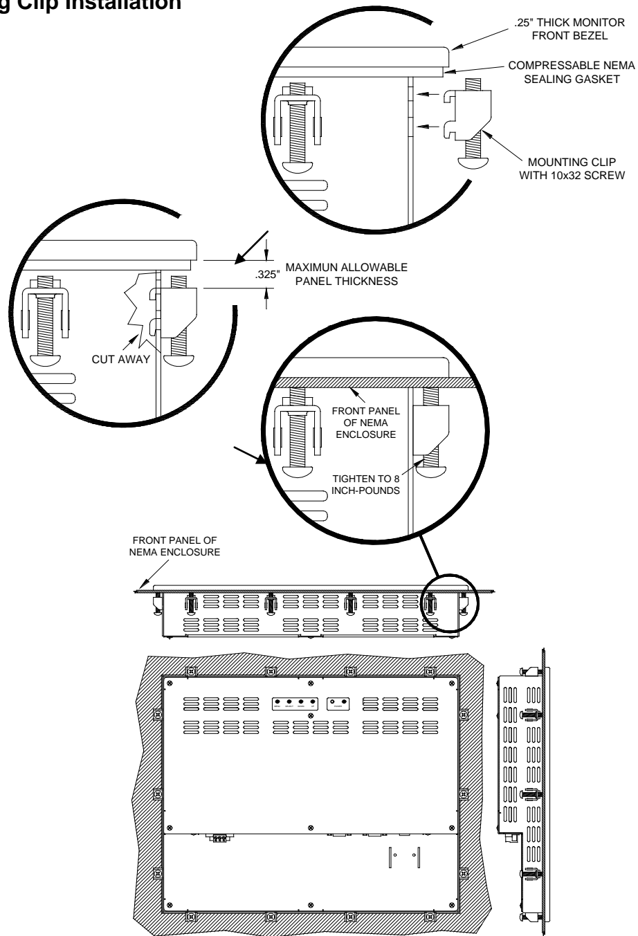
REAR VIEW OF PANEL MOUNTED @PC
