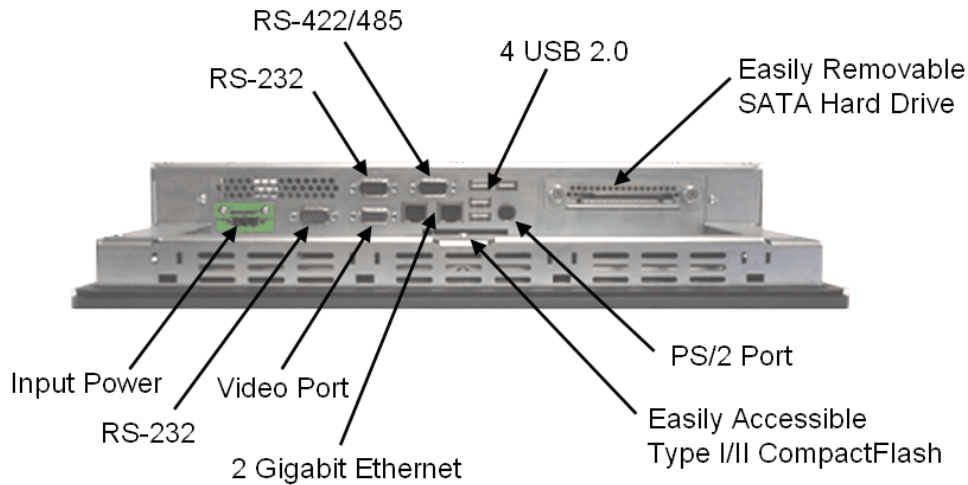
Figure 2.0: ePC Series I/O configuration
