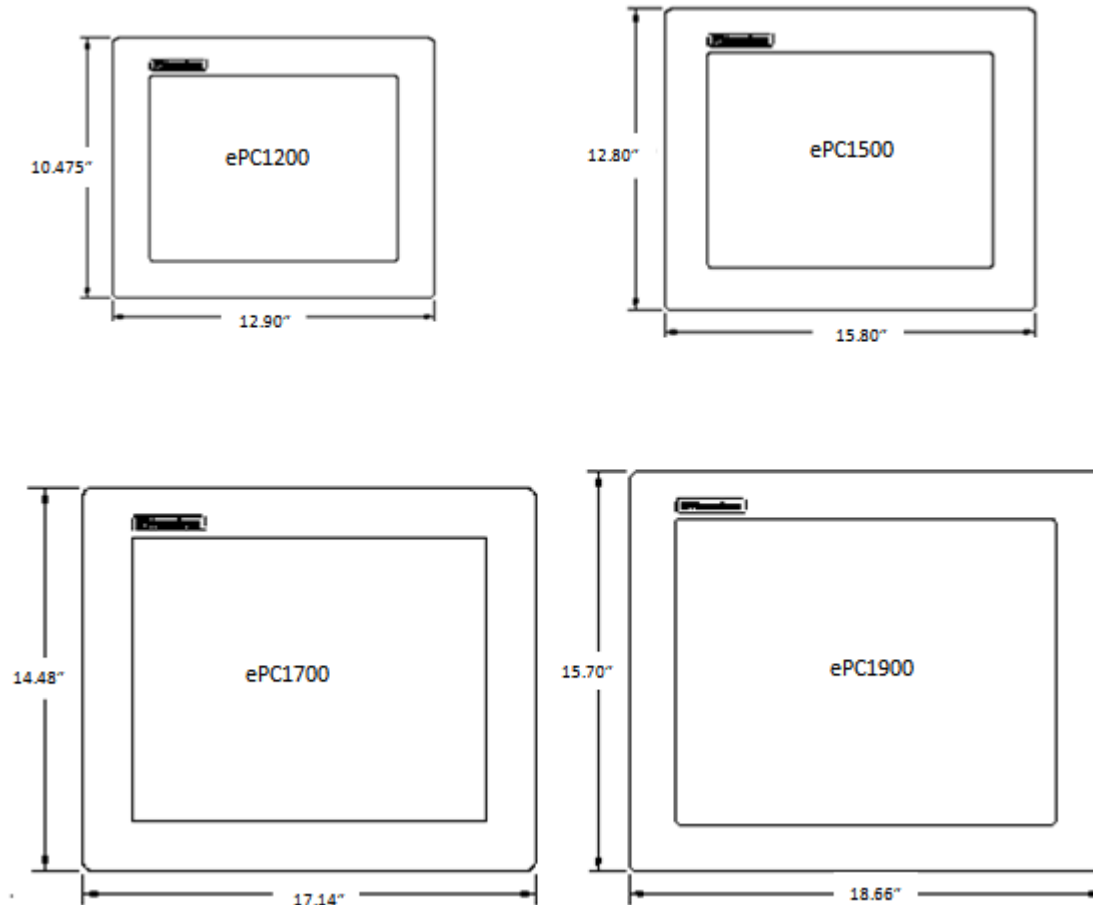
Figure 1.0: ePC Series Front Panel Comparison
