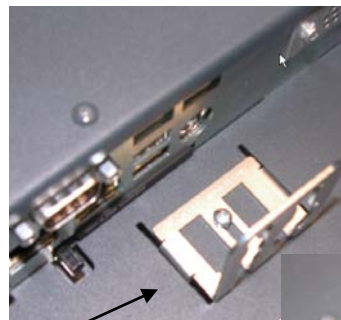
ePC-Series USB Retention Bracket
