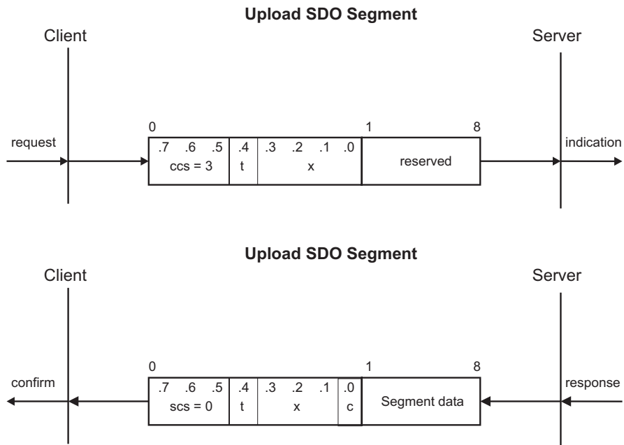
Fig. 5-7: Upload SDO Segment
