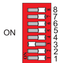
Fig. 3-11: Setting the Baud rate 125 kB
