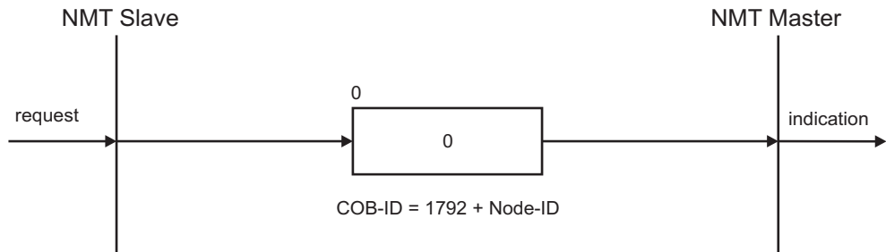
Fig. 5-18:Bootup Protocol
