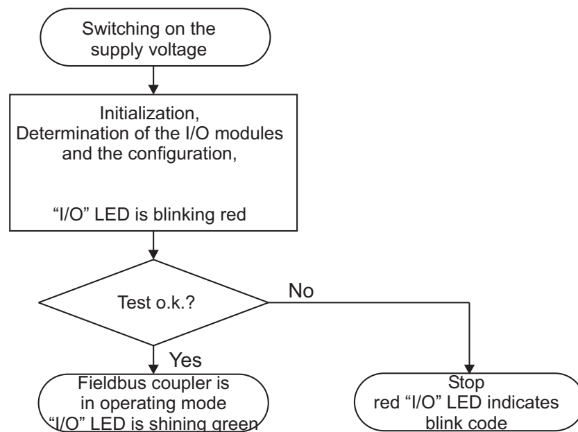
Fig. 3-8: Operating I/O-System - Power on
