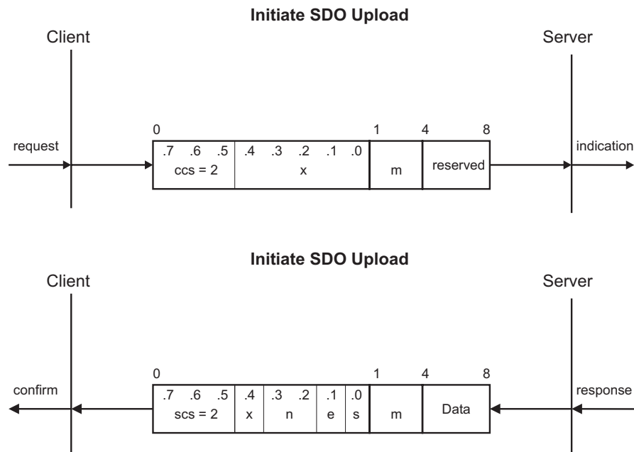
Fig. 5-6: Initiate SDO Upload
