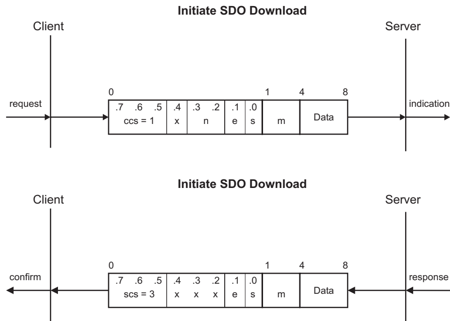
Fig. 5-4:Initiate SDO
