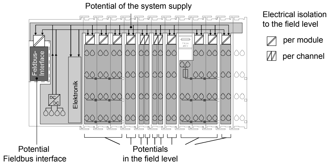
Fig. 2-10: Isolation
