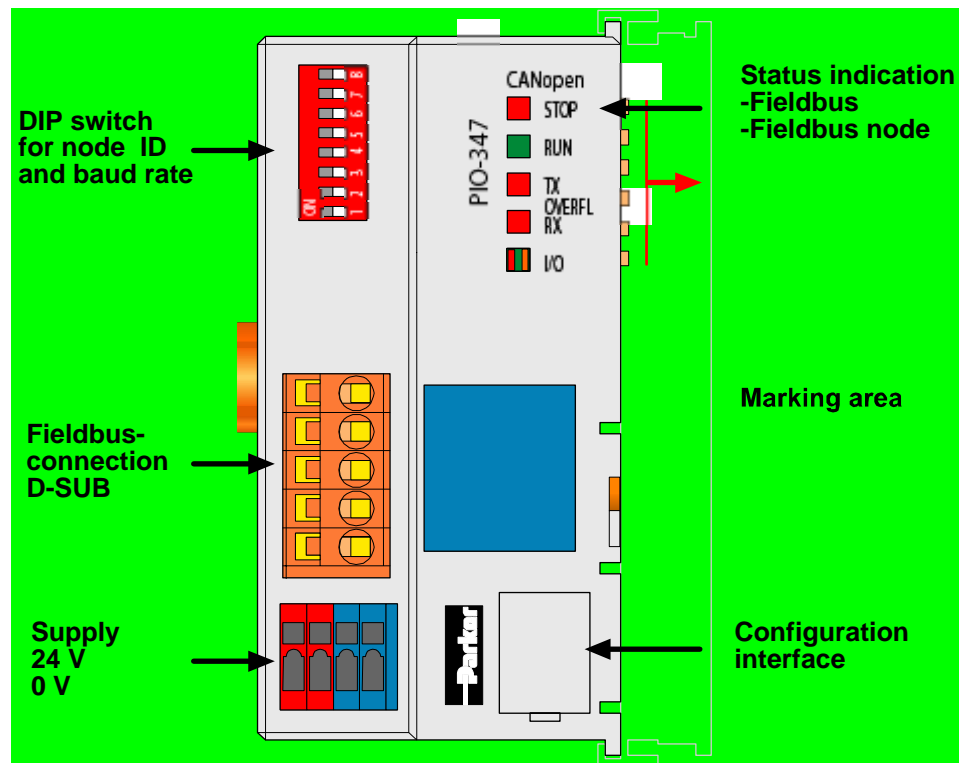
Fig. 3-1: ECO fieldbus coupler CANopen
