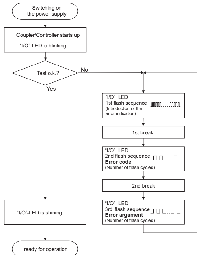
Fig. 3-15: Signalling the LED's node status
