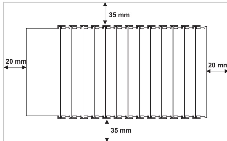
Fig. 2-4: Spacing
