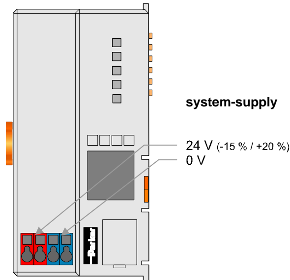
Fig. 2-11: I/O-System Supply
