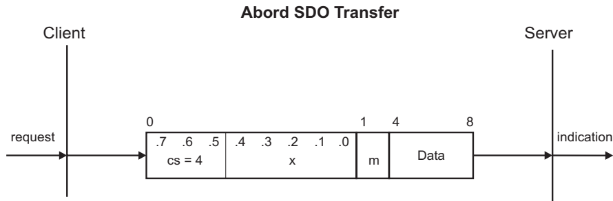
Fig. 5-8:Abort SDO Transfer
