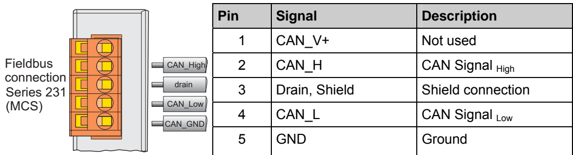
Fig. 3-3: Pin assignment for fieldbus connection
