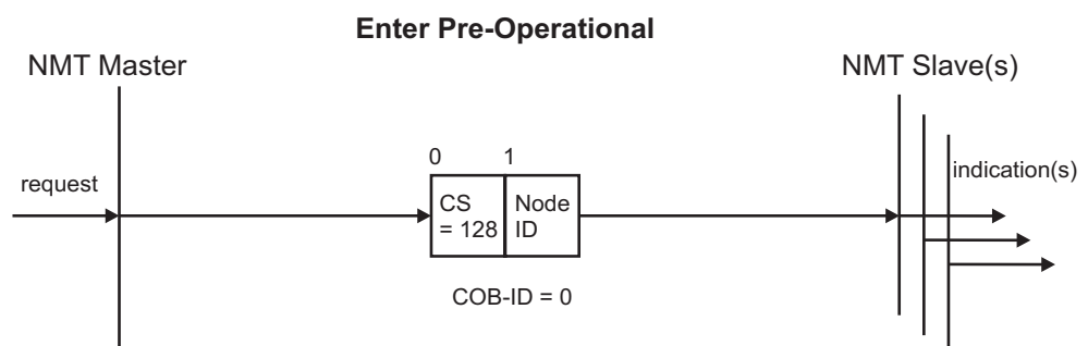
Fig. 5-14:Enter PRE-OPERATIONAL
