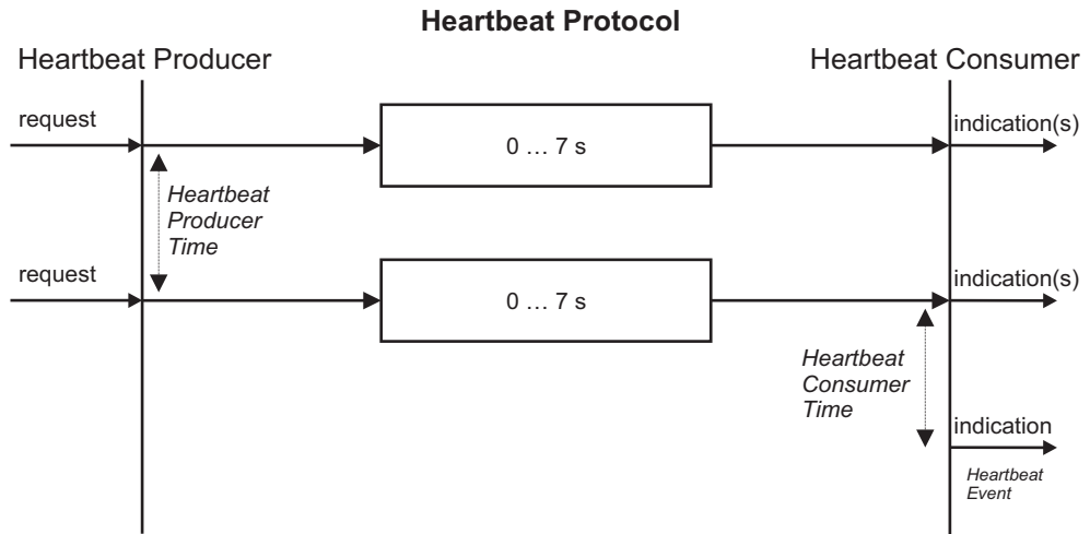
Fig. 5-17:Heartbeat Protocol
