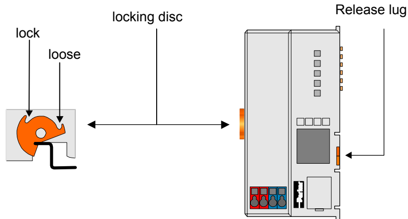
Fig. 2-5: Coupler and unlocking lug
