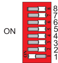
Fig. 3-6: Setting of station (node) address
