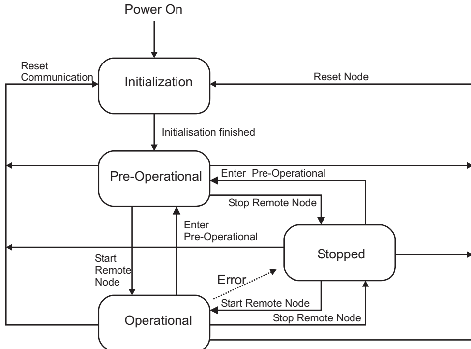
Fig. 5-11: State diagram of the fieldbus couple
