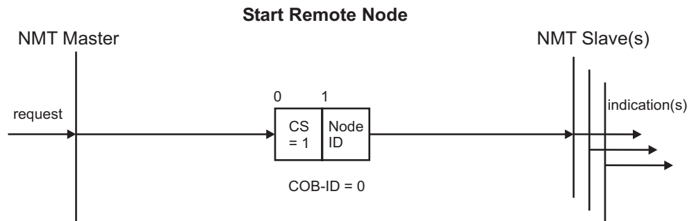
Fig. 5-12:Start Remote Node
