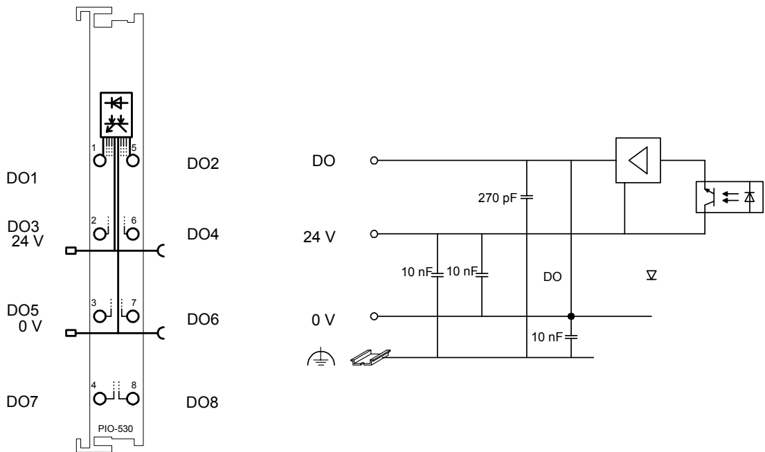
Fig. 4.8.4-1: 8-Channel Digital Output Module PIO-530
