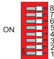
Fig. 3-10: All DIP switches to "OFF" for checking and setting the Baud rate
