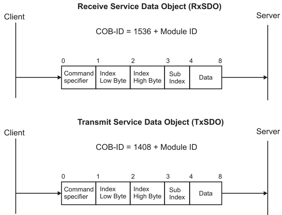
Fig. 5-3:SDO Protocol
