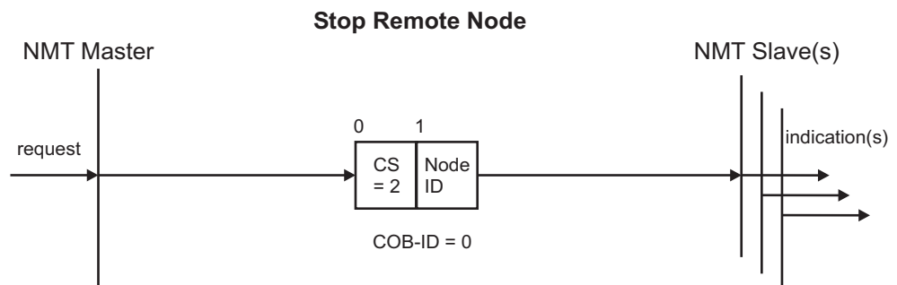
Fig. 5-13:Stop Remote Node
