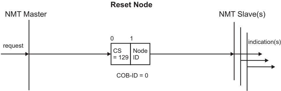
Fig. 5-15:Reset Node
