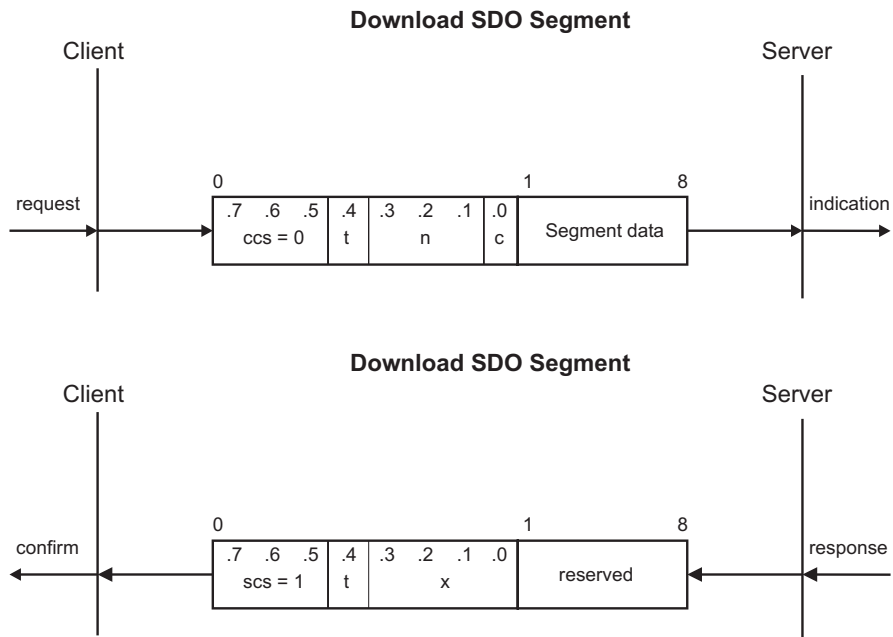
Fig. 5-5:Download SDO Segment
