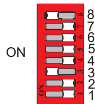
Fig. 3-7: Example: Saving the baud rate 125 kB
