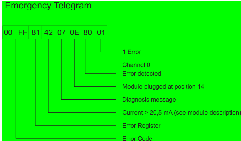
Fig. 5-20: Design Emergency Message 1
