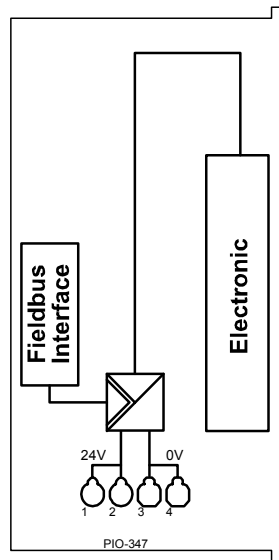
Fig. 3-2: Device supply
