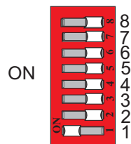
Fig. 3-13: Setting the module ID 1
