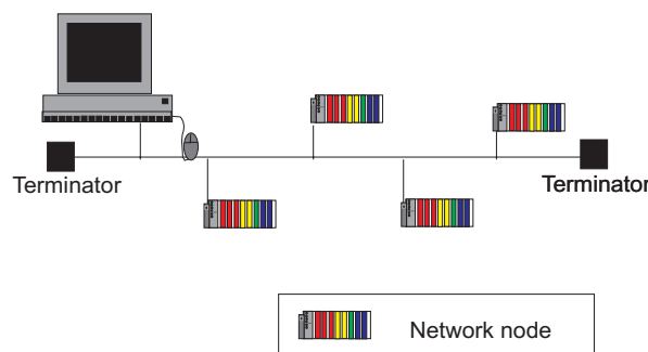
Fig. 5-2: Bus topology of a CANopen network
