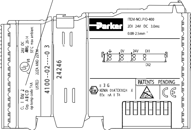
Fig. 6-2: Example for lateral labeling of bus modules (PIO-400, 2 channel digital input module 24 V DC)
