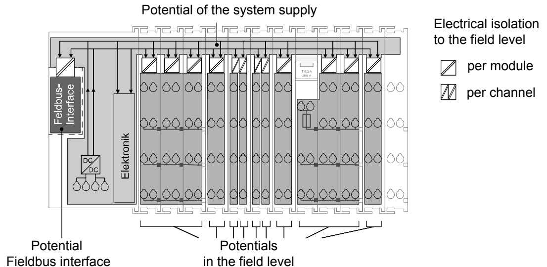
Fig. 2-10: Isolation
