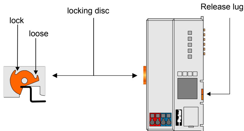
Fig. 2-5: Coupler and unlocking lug
