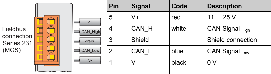
Fig. 3-3: Fieldbus connection, MCS
