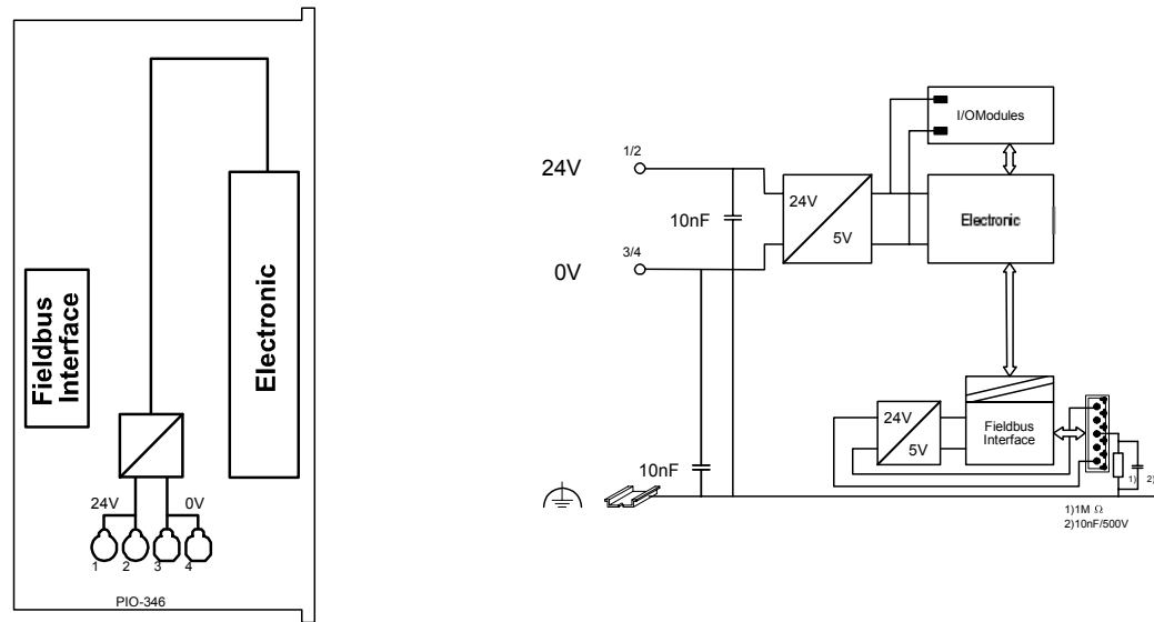
Fig. 3-2: Device supply
