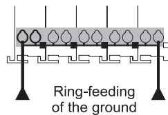
Fig. 2-14: Ring-feeding
