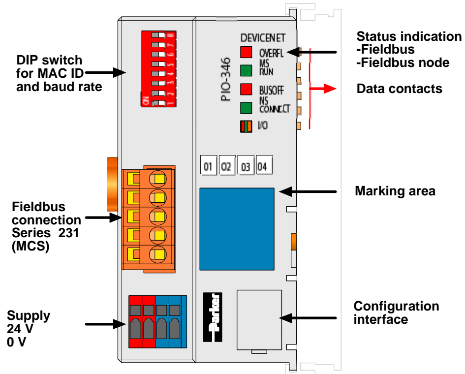
Fig. 3-1: ECO fieldbus coupler DeviceNet
