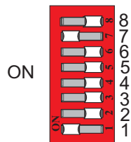
Fig. 3-7: Example: Setting the baud rate 250 kBaud (DIP 7 = ON) on a station (node) with the address MAC ID 1.
