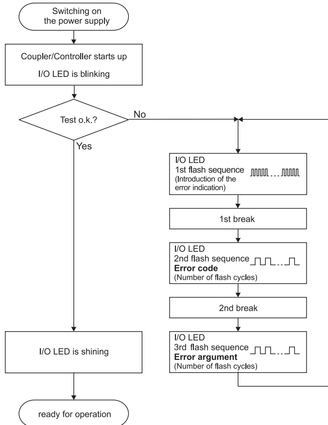
Fig. 3-13: Signalling the LED's node status
