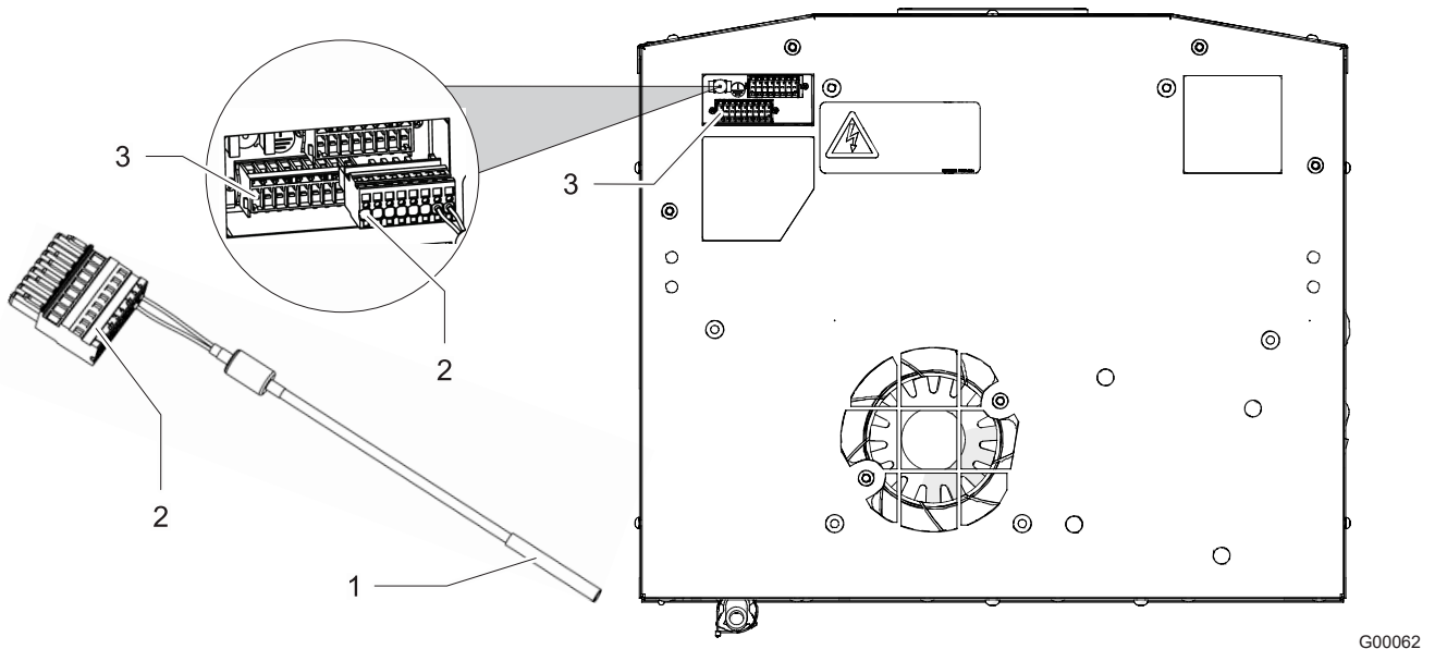
Fig. 23: Temperature sensor - TS2
