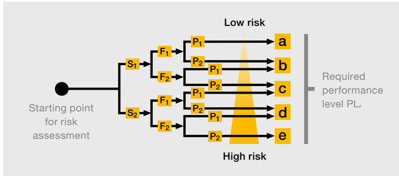
Risk analysis in accordance with EN ISO 13849-1
