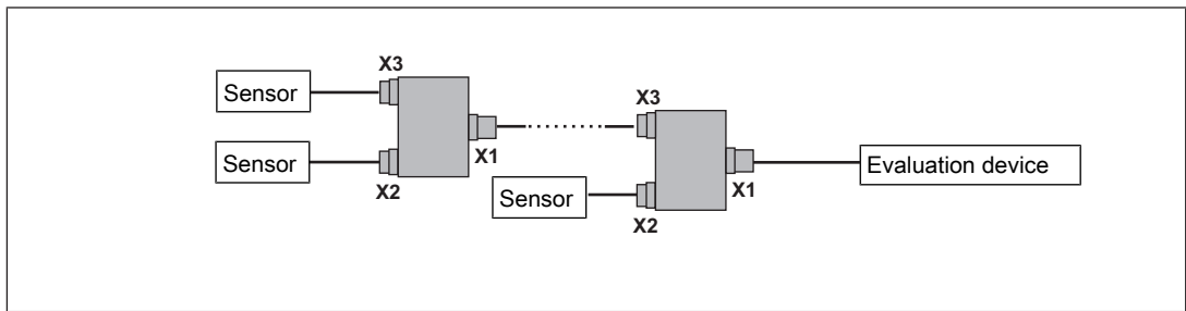
Fig.: Connection PSEN Y junction M8 cable channel (order no. 540318)
