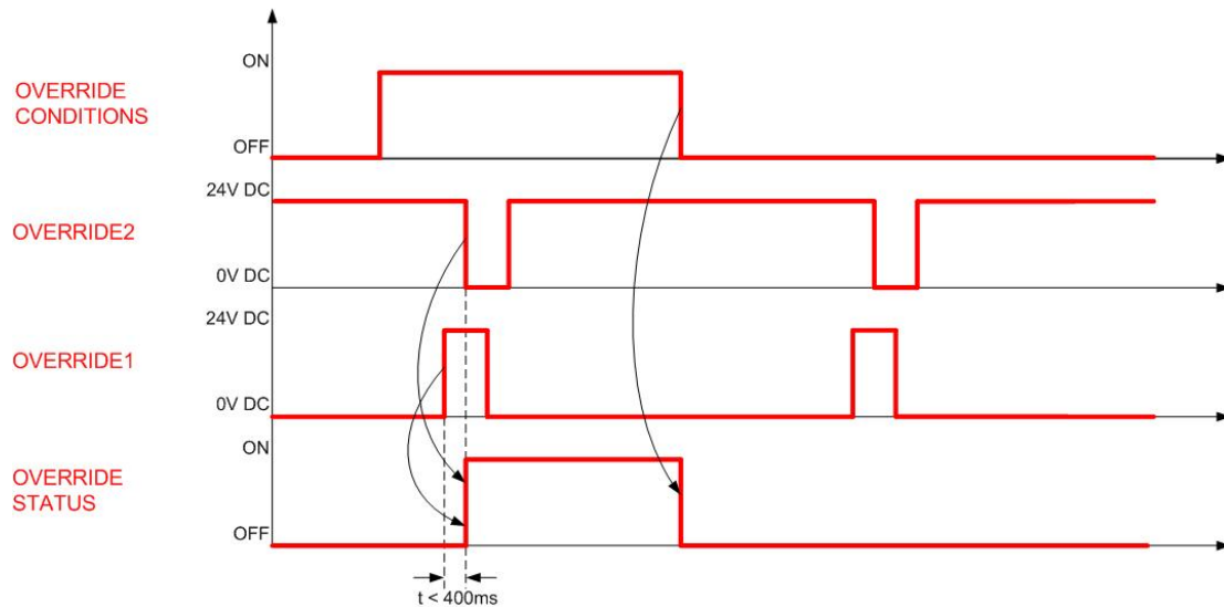
Fig. 48 – Override timings (activated by edge)
