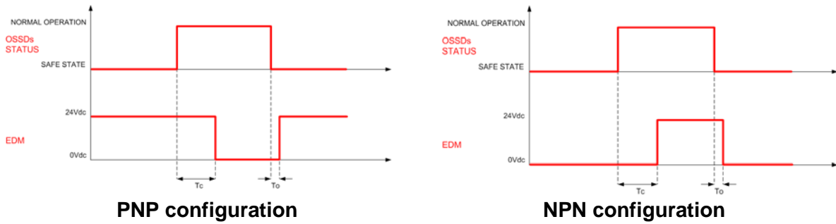
Fig. 36 – EDM timings
