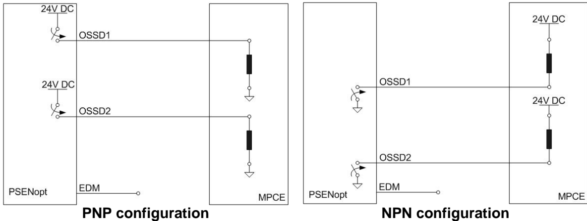
Fig. 37 – EDM connections
