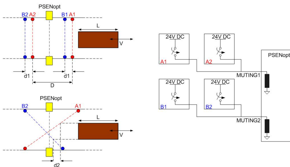
Fig. 43 – T-Muting connection
