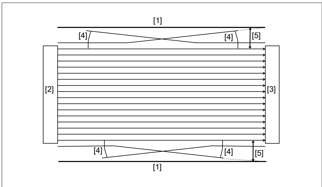
Fig.: Interference with the function of the safety light curtain due to reflective surfaces – top view
