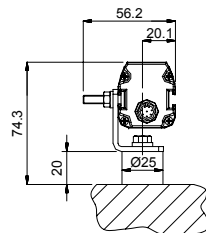
Standard bracket (Bracket kit PSEN 4) + antivibration support (Bracket kit PSEN 4 anti vibr.)
