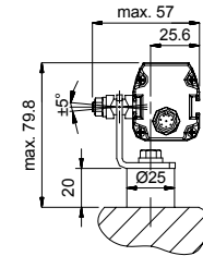
Standard bracket (Bracket kit PSEN 4) + orientable support (Bracket kit PSEN 4 adjust.) + antivibration support (Bracket kit PSEN 4 anti vibr.)
