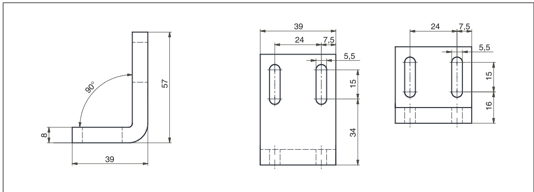
Fig.: Mounting bracket for sliding gate (see Accessories [29] )
