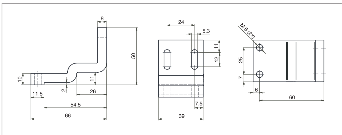
Fig.: Mounting bracket for swing gate (see Accessories [29] )
