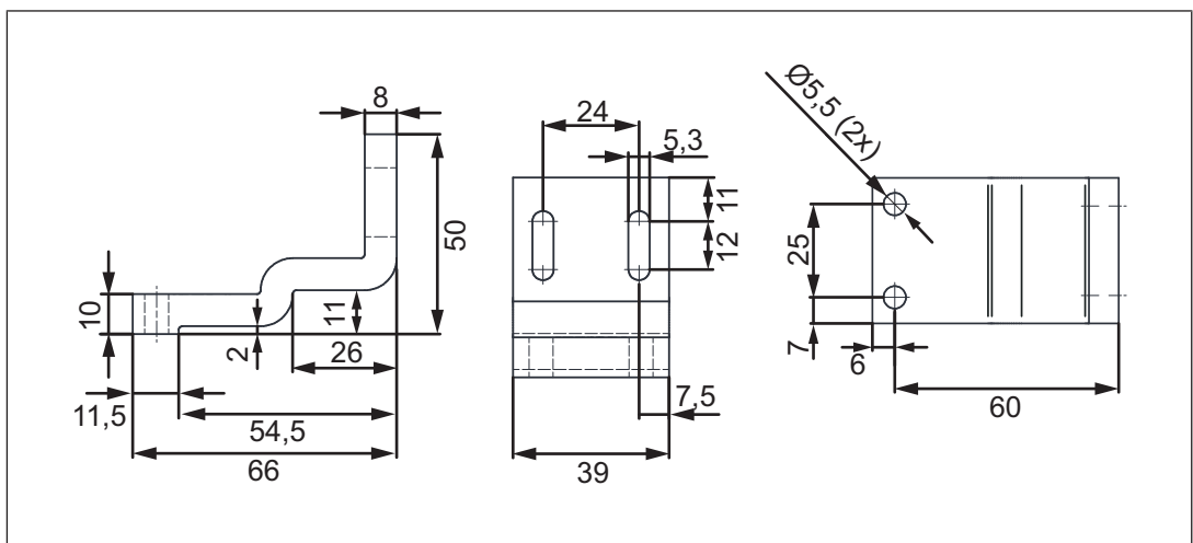
Fig.: Mounting bracket for swing gate (see Accessories [36])
