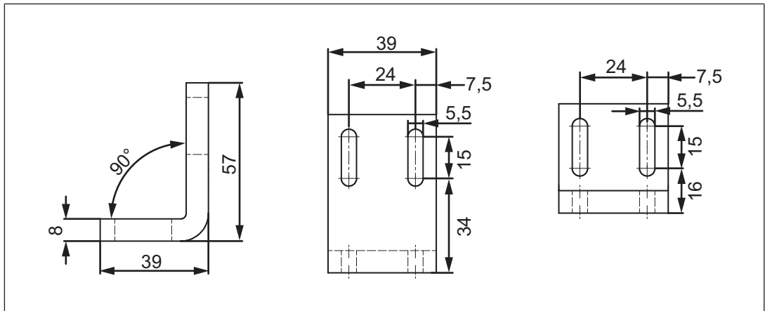
Fig.: Mounting bracket for sliding gate (see Accessories [36])
