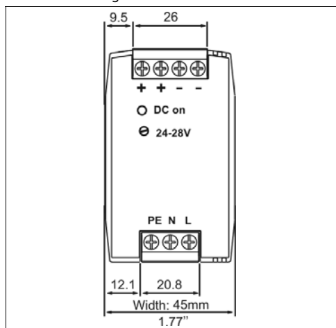
Fig. 20-1 Front view
