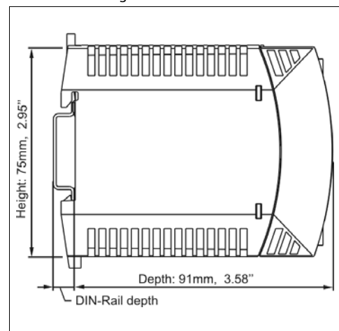
Fig. 20-2 Side view
