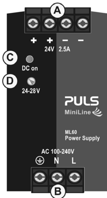
Fig. 10-1 Front side
