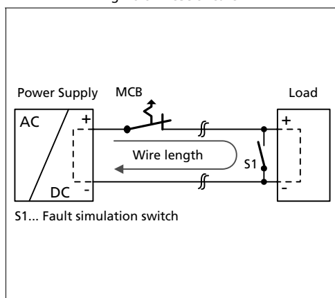
Fig. 25-5 Test circuit
