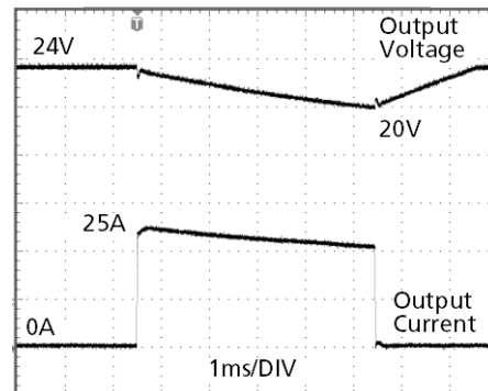
25A Peak load (resistive) for 5ms Output voltage dips from 24V to 20V.
