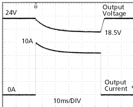
10A Peak load (resistive) for 50ms Output voltage dips from 24V to 18.5V.
